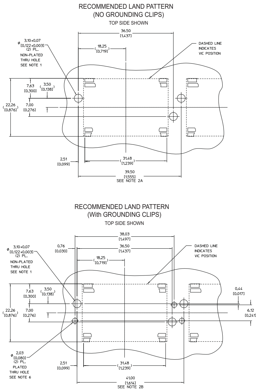
Figure 19 — Hole location for push pin heat sink relative to V-I Chip
