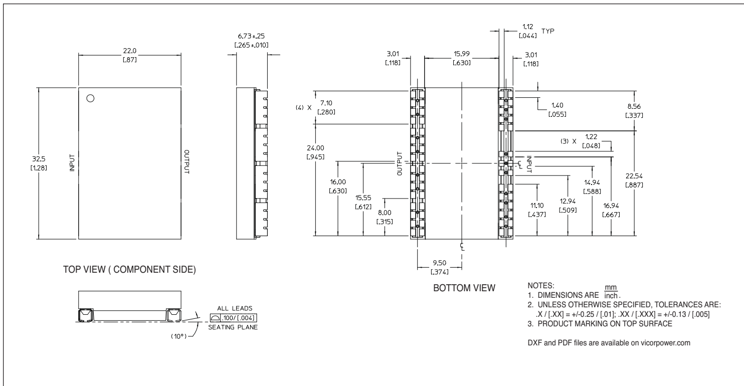
Figure 10 — VTM™ module J-Lead mechanical outline; Onboard mounting
