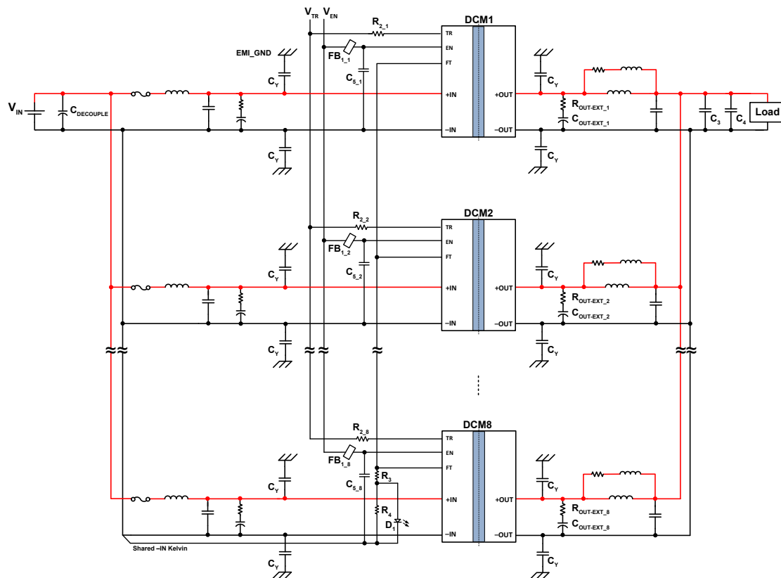
Figure 26 — DCM paralleling configuration circuit 1
