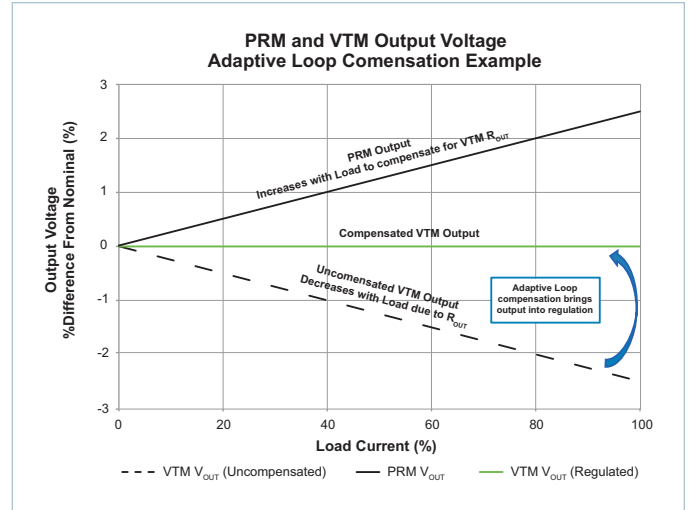
Figure 27 — Adaptive Loop Compensation Illustration
