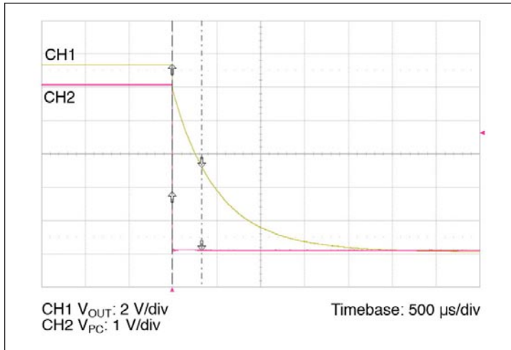
Figure 13 – PC disable waveform, 48 V IN , 500 μF C OUT full load
