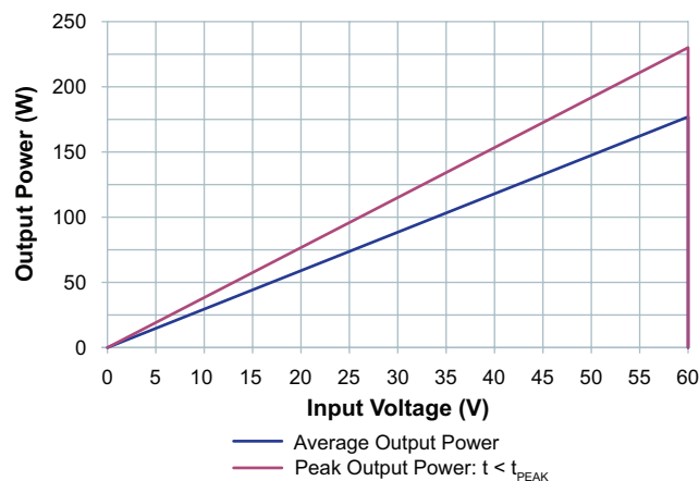
Figure 2 — Specified electrical operating area, R_{OUT} max hot
