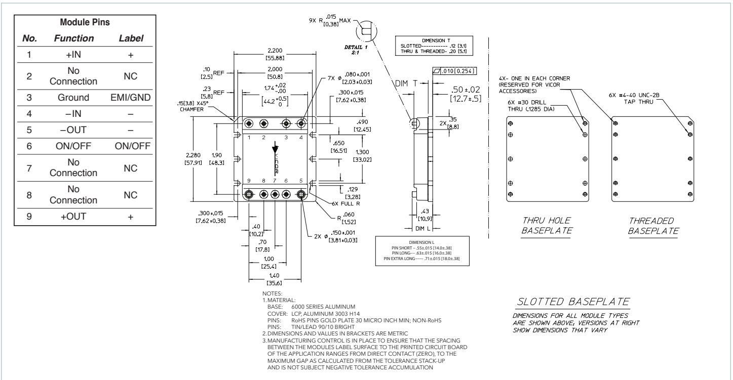
Figure 8 — Mechanical diagram
