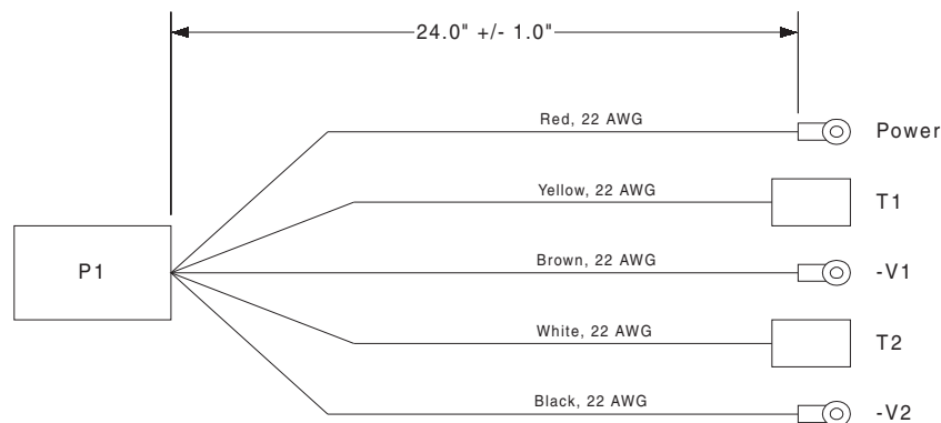
Figure 3. Cable Drawing
