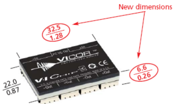
New V•I Chip package (Date code 0635 and later)
