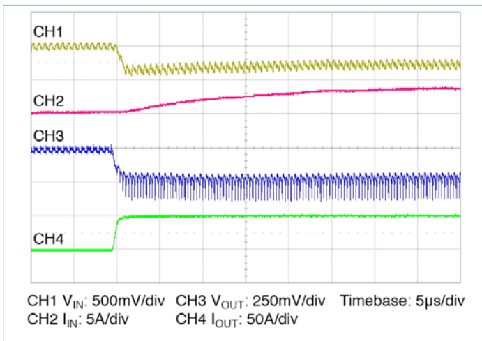
Figure 14 — 0 – 50A transient response: C_{IN} = 330\mu\text{F} , I_{IN} measured prior to C_{IN} , no external C_{OUT}
