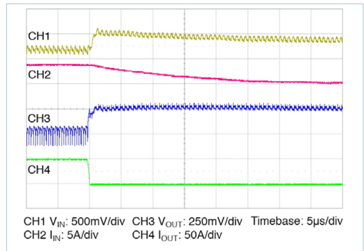
Figure 15 — 50 – 0A transient response: C_{IN} = 330\mu\text{F} , I_{IN} measured prior to C_{IN} , no external C_{OUT}
