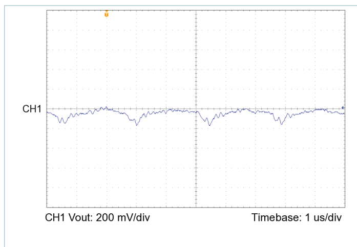
Figure 18 — Output voltage ripple, V_{IN} = 100\text{V} , V_{OUT} = 3.3\text{V} , C_{OUT\_EXT} = 470\mu\text{F} , R_{LOAD} = 0.270\Omega
