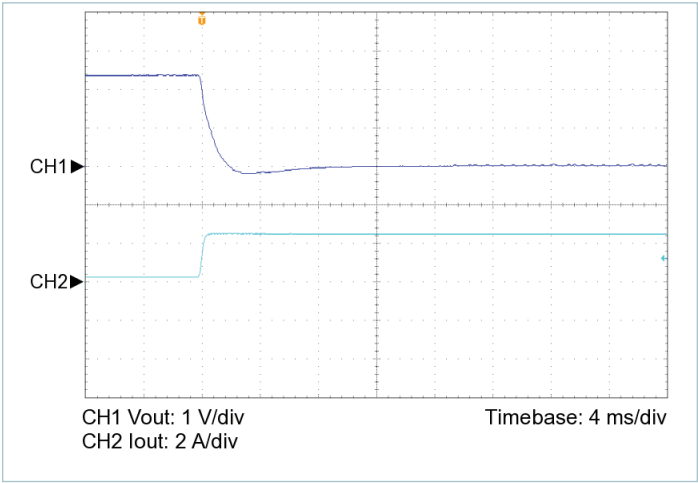
Figure 23 — 10 – 100% load transient response, V_{IN} = 100\text{V} , nominal trim, C_{OUT\_EXT} = 220\mu\text{F}
