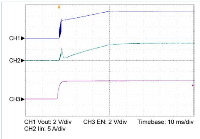
Figure 20 — Start up from EN, V_{IN} = 24\text{V} , C_{OUT\_EXT} = 20000\mu\text{F} , R_{LOAD} = 0.139\Omega
