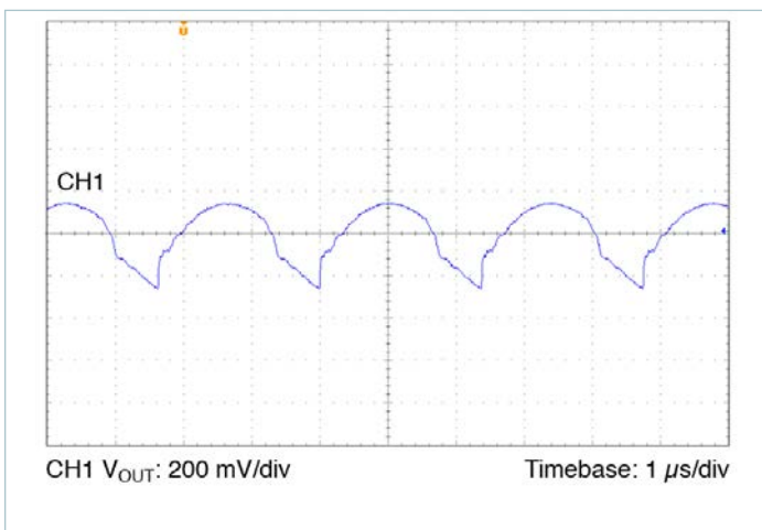
Figure 22 — Output voltage ripple, V_{IN} = 24\text{V} , V_{OUT} = 5.0\text{V} , C_{OUT\_EXT} = 1000\mu\text{F} , R_{LOAD} = 0.139\Omega
