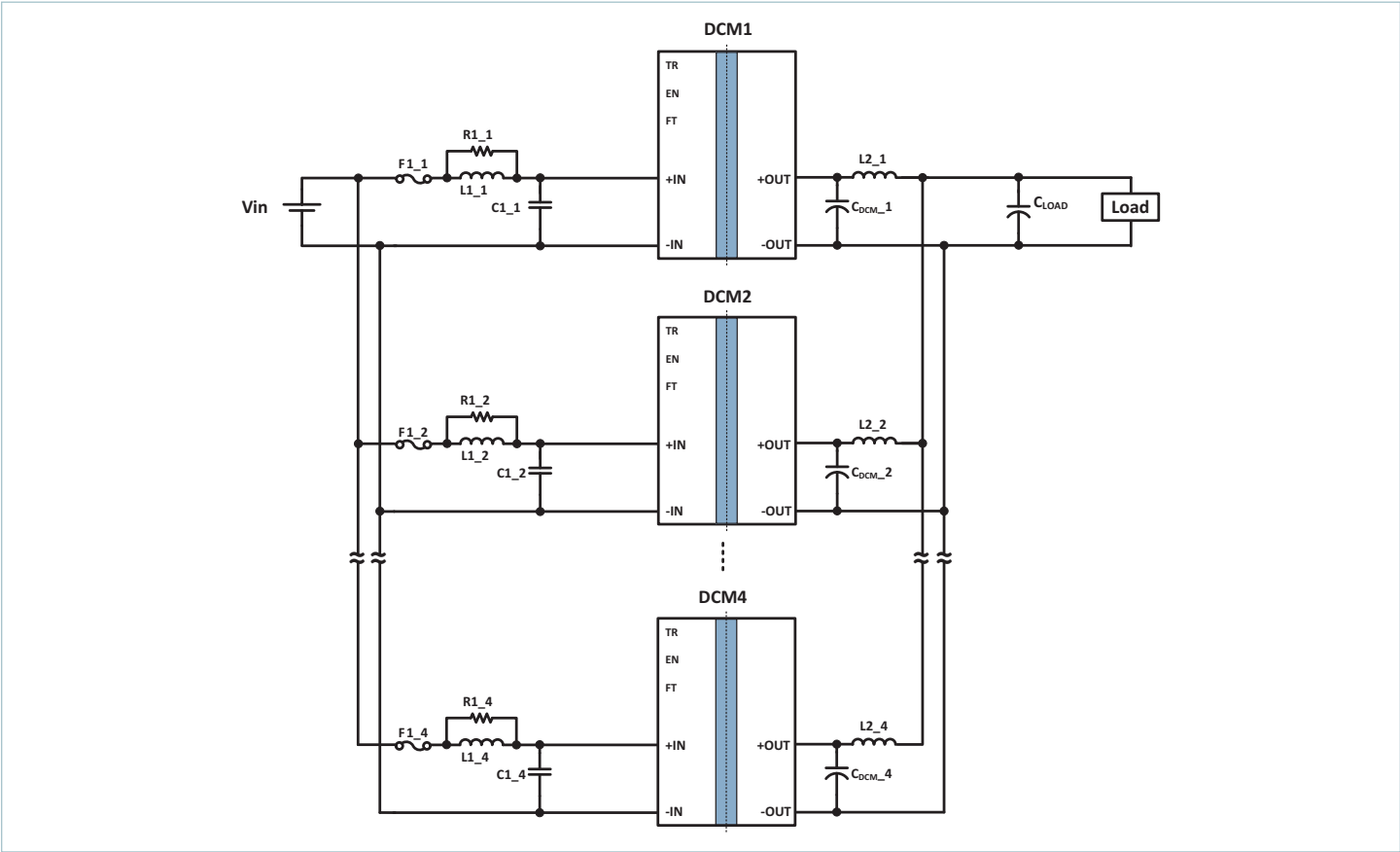
Typical Application 1: DCM3623x40R53A6yzz in an array of four units
