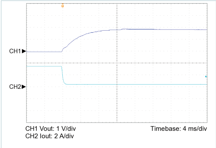
Figure 7 — 100% to 10% load transient response, V_{IN} = 30\text{ V} , nominal trim, C_{OUT\_EXT} = 220\text{ }\mu\text{F}
