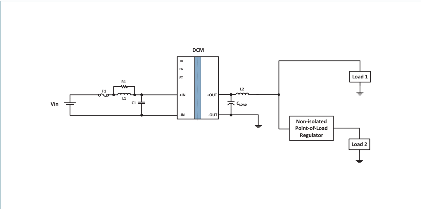
Typical Application 2: Single DCM3623x40R53A6yzz, to a non-isolated regulator, and direct to load
