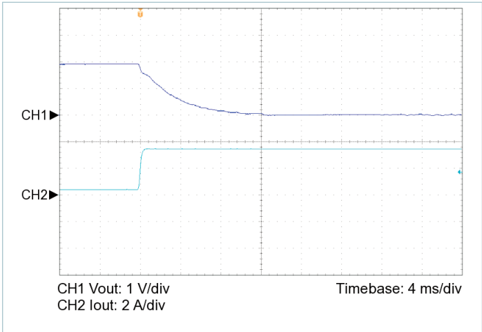
Figure 8 — 10% to 100% load transient response, V_{IN} = 30\text{ V} , nominal trim, C_{OUT\_EXT} = 220\text{ }\mu\text{F}
