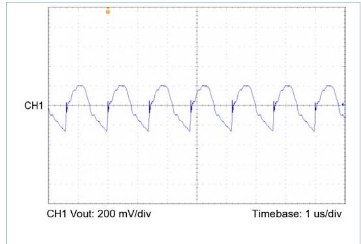
Figure 18 — Output voltage ripple, V_{IN} = 28\text{V} , V_{OUT} = 12.0\text{V} , C_{OUT\_EXT} = 1000\mu\text{F} , R_{LOAD} = 0.450\Omega
