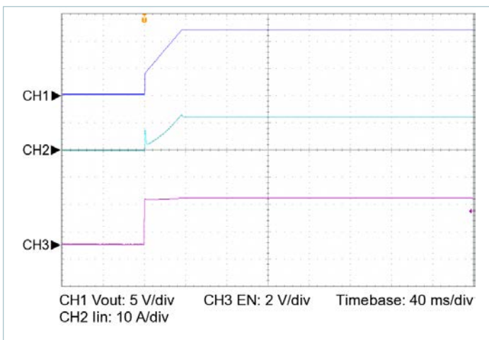
Figure 19 — Start up from EN, V_{IN} = 28\text{V} , C_{OUT\_EXT} = 10000\mu\text{F} , R_{LOAD} = 0.450\Omega
