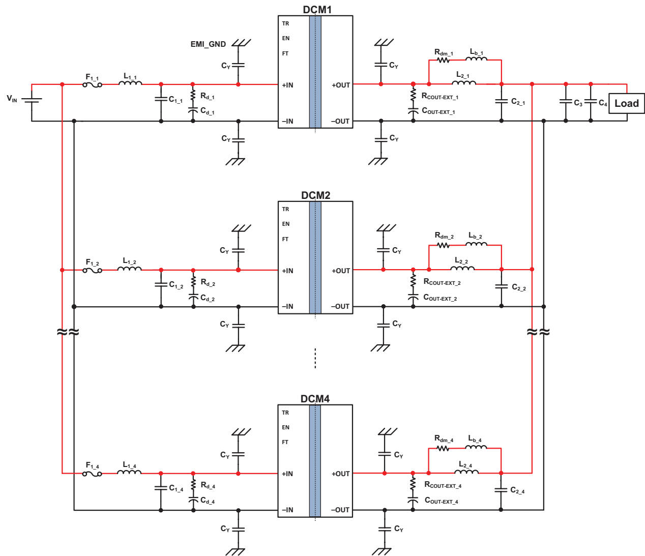
Typical application 1: DCM3623x50M17C2yzz in an array of four units
