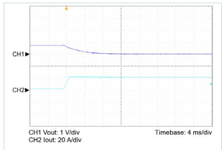
Figure 8 — 10 – 100% load transient response, V_{IN} = 28\text{V} , nominal trim, C_{OUT\_EXT} = 680\mu\text{F}
