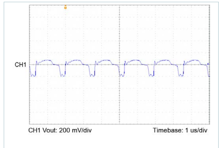
Figure 18 — Output voltage ripple, V_{IN} = 30\text{V} , V_{OUT} = 5.0\text{V} , C_{OUT\_EXT} = 1000\mu\text{F} , R_{LOAD} = 0.313\Omega
