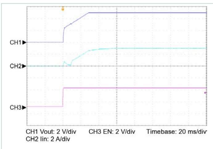
Figure 19 — Start up from EN, V_{IN} = 30\text{V} , C_{OUT\_EXT} = 10000\mu\text{F} , R_{LOAD} = 0.313\Omega
