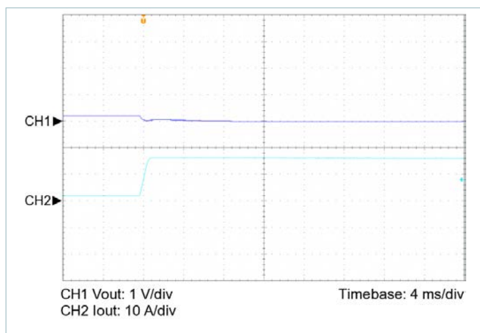
Figure 8 — 10 – 100% load transient response, V_{IN} = 30\text{V} , nominal trim, C_{OUT\_EXT} = 1000\mu\text{F}
