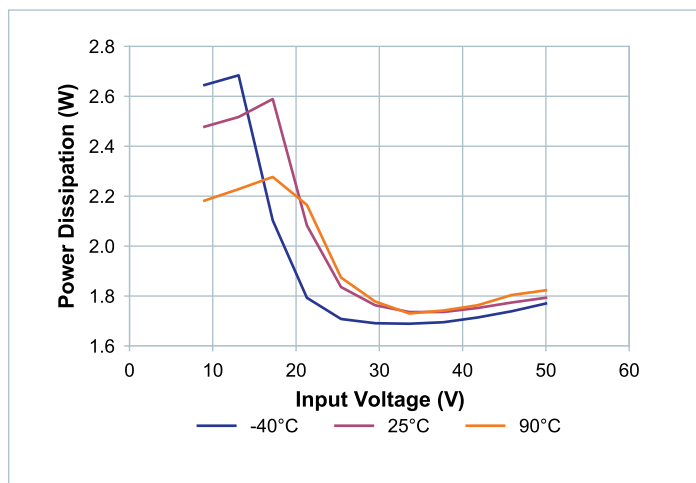
Figure 4 — No-load power dissipation vs. V_{INr} at nominal trim
