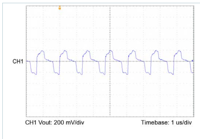
Figure 18 — Output voltage ripple, V_{IN} = 30\text{V} , V_{OUT} = 12.0\text{V} , C_{OUT\_EXT} = 1000\mu\text{F} , R_{LOAD} = 0.896\Omega
