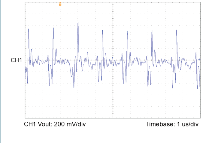
Figure 16 — Output voltage ripple, V_{IN} = 42\text{ V} , V_{OUT} = 15.0\text{ V} , C_{OUT\_EXT} = 1000\text{ }\mu\text{F} , R_{LOAD} = 2.778\text{ }\Omega
