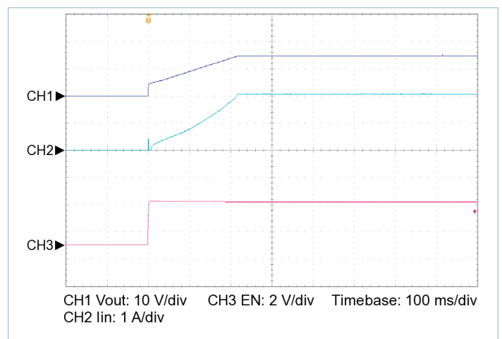
Figure 14 — Startup from EN, V_{IN} = 42\text{ V} , C_{OUT\_EXT} = 10000\text{ }\mu\text{F} , R_{LOAD} = 2.778\text{ }\Omega
