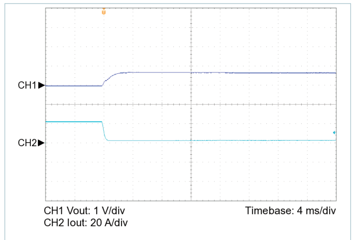
Figure 7 — 100% to 10% load transient response, V_{IN} = 110\text{ V} , nominal trim, C_{OUT\_EXT} = 1000\ \mu\text{F}
