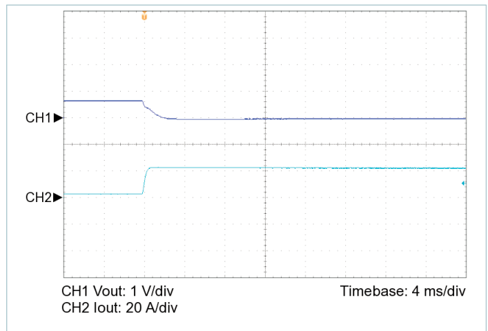
Figure 8 — 10% to 100% load transient response, V_{IN} = 110\text{ V} , nominal trim, C_{OUT\_EXT} = 1000\ \mu\text{F}
