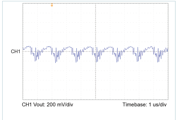
Figure 19 — Output voltage ripple, V_{IN} = 110\text{ V} , V_{OUT} = 13.8\text{ V} , C_{OUT\_EXT} = 1000\text{ }\mu\text{F} , R_{LOAD} = 0.633\text{ }\Omega
