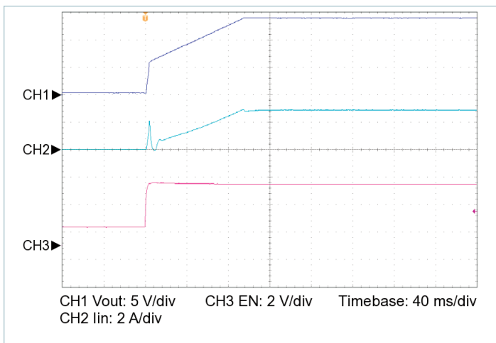
Figure 17 — Startup from EN, V_{IN} = 110\text{ V} , C_{OUT\_EXT} = 20000\text{ }\mu\text{F} , R_{LOAD} = 0.633\text{ }\Omega
