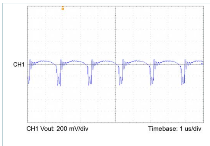
Figure 18 — Output voltage ripple, V_{IN} = 100\text{V} , V_{OUT} = 3.3\text{V} , C_{OUT\_EXT} = 1000\mu\text{F} , R_{LOAD} = 0.136\Omega
