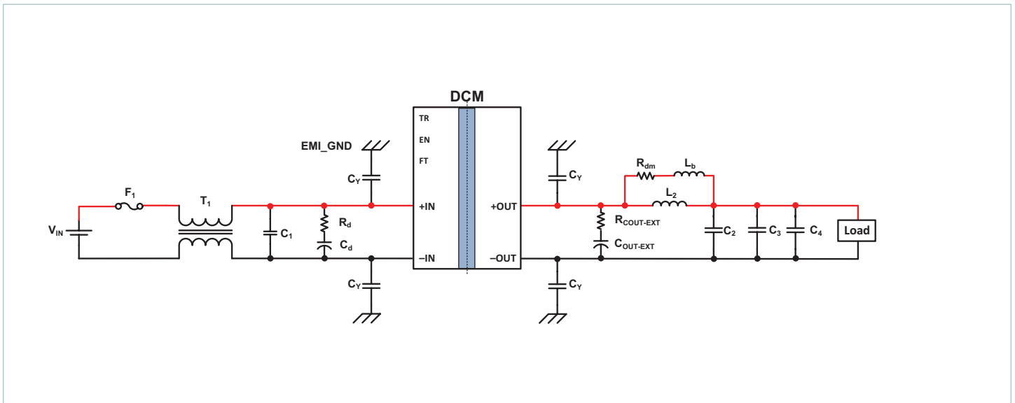
Typical application 2: single DCM3623xA5N0480y7z with common- and differential-mode input filters
