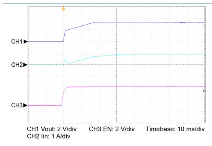
Figure 19 — Start up from EN, V_{IN} = 100\text{V} , C_{OUT\_EXT} = 20000\mu\text{F} , R_{LOAD} = 0.136\Omega
