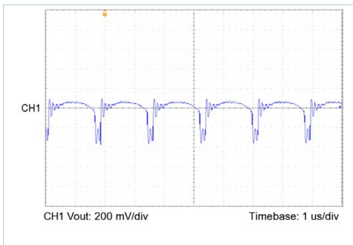
Figure 22 — Output voltage ripple, V_{IN} = 100\text{V} , V_{OUT} = 3.3\text{V} , C_{OUT\_EXT} = 1000\mu\text{F} , R_{LOAD} = 0.136\Omega
