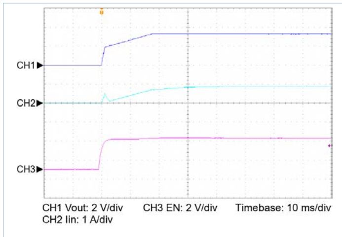
Figure 20 — Start up from EN, V_{IN} = 100\text{V} , C_{OUT\_EXT} = 20000\mu\text{F} , R_{LOAD} = 0.136\Omega
