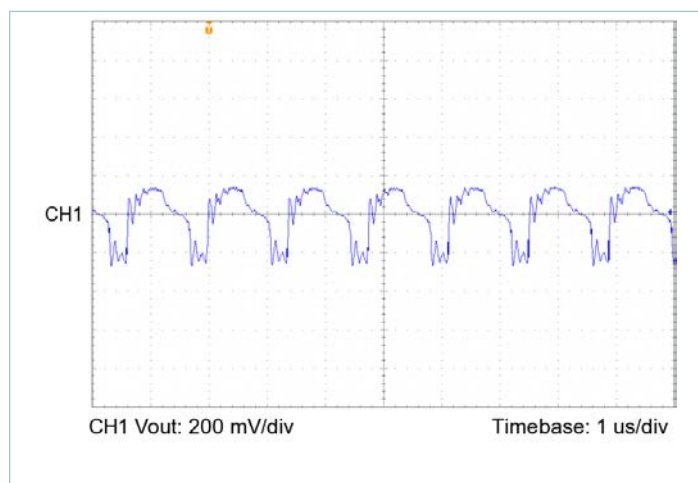
Figure 22 — Output voltage ripple, V_{IN} = 100\text{V} , V_{OUT} = 12.0\text{V} , C_{OUT\_EXT} = 1000\mu\text{F} , R_{LOAD} = 0.600\Omega
