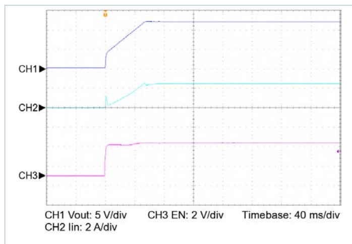
Figure 20 — Start up from EN, V_{IN} = 100\text{V} , C_{OUT\_EXT} = 20000\mu\text{F} , R_{LOAD} = 0.600\Omega
