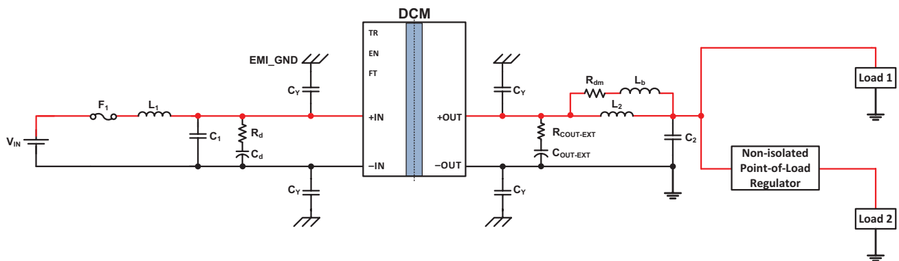
Typical application 2: single DCM3623xA5N13B4yzz, to a non-isolated regulator, and direct to load
