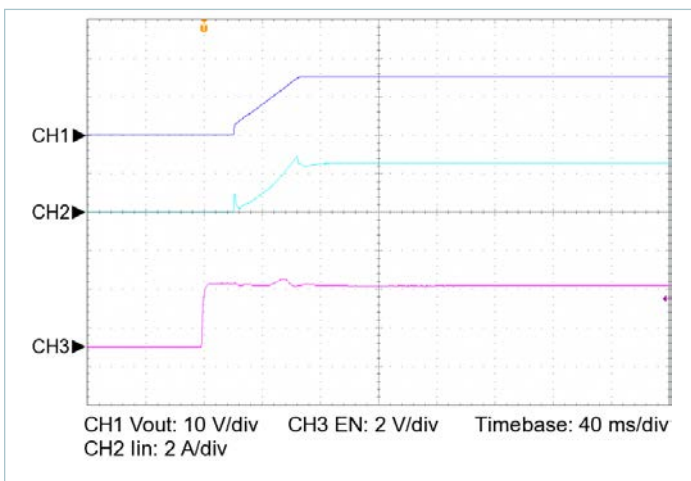
Figure 19 — Start up from EN, V_{IN} = 100\text{V} , C_{OUT\_EXT} = 20000\mu\text{F} , R_{LOAD} = 0.938\Omega
