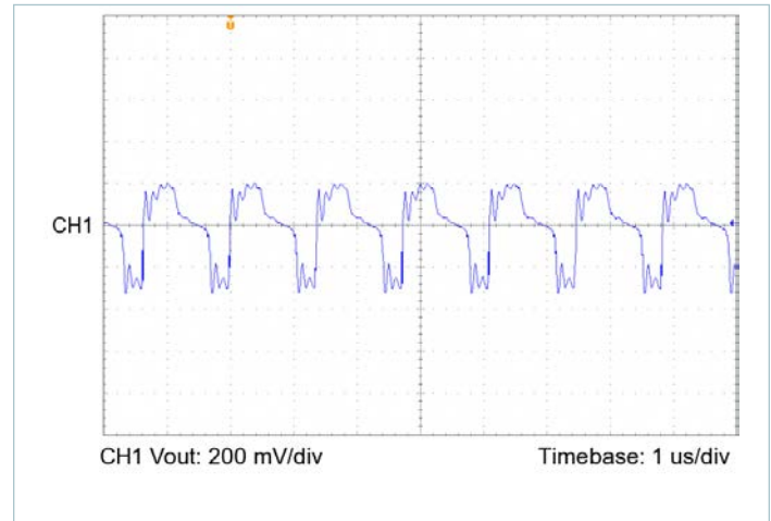
Figure 18 — Output voltage ripple, V_{IN} = 100\text{V} , V_{OUT} = 15.0\text{V} , C_{OUT\_EXT} = 1000\mu\text{F} , R_{LOAD} = 0.938\Omega
