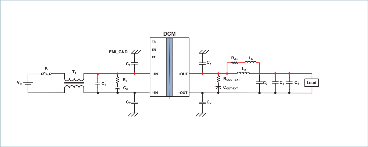
Typical application 2: single DCM3623xA5N17B4y7z with common- and differential-mode input filters
