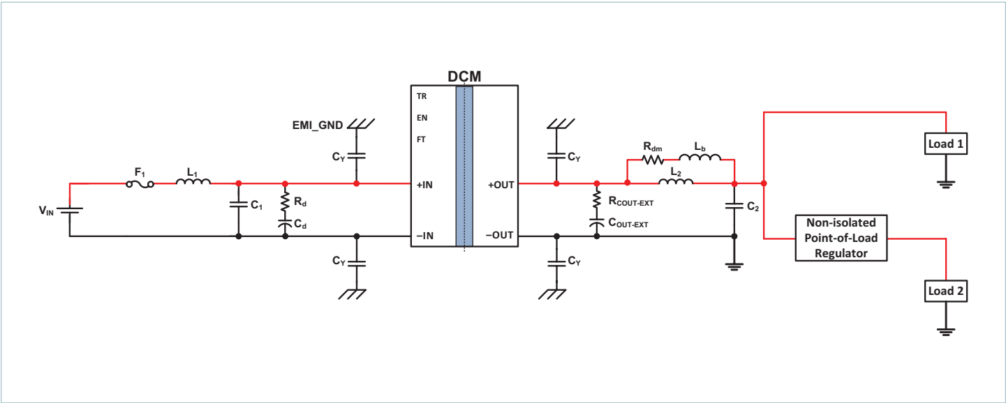
Typical application 1: single DCM3623xA5N17B4y7z to a non-isolated regulator and direct to load
