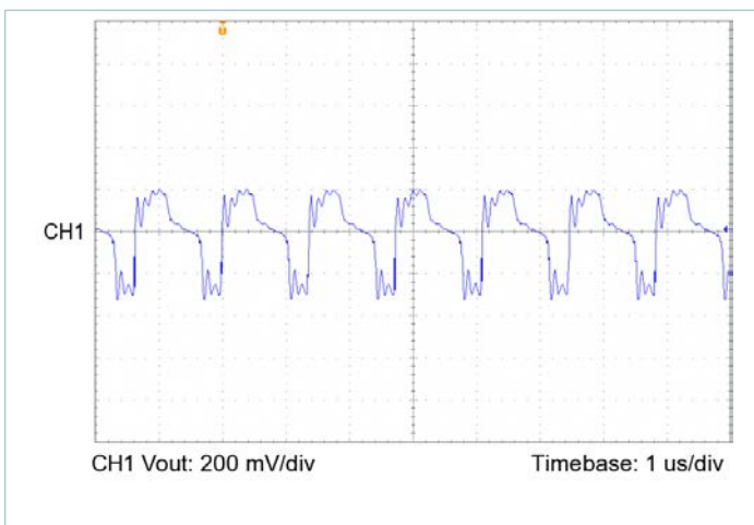
Figure 22 — Output voltage ripple, V_{IN} = 100\text{V} , V_{OUT} = 15.0\text{V} , C_{OUT\_EXT} = 1000\mu\text{F} , R_{LOAD} = 0.938\Omega
