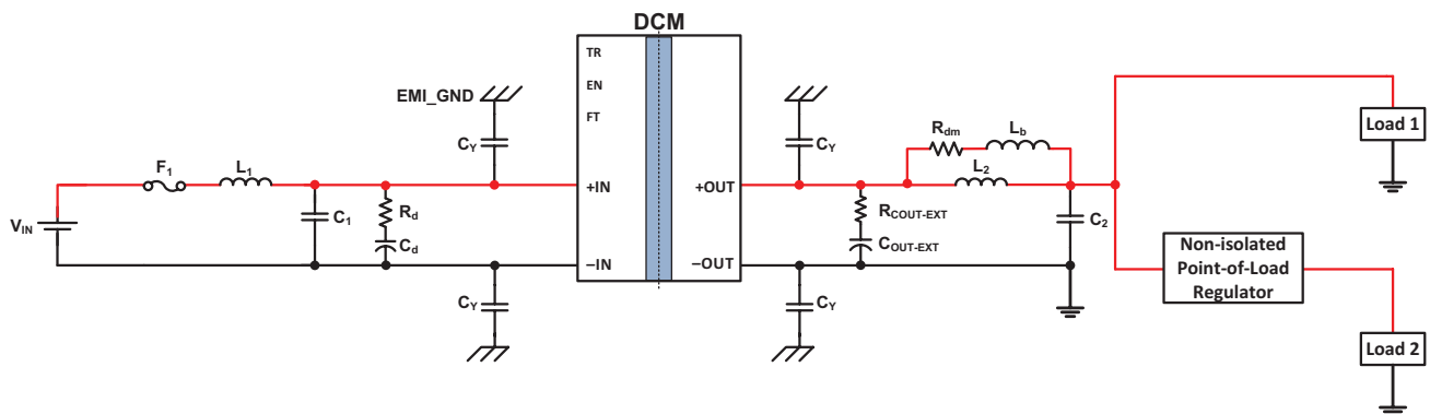
Typical application 2: single DCM3623xA5N17B4yzz, to a non-isolated regulator, and direct to load
