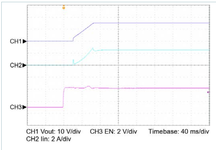
Figure 20 — Start up from EN, V_{IN} = 100\text{V} , C_{OUT\_EXT} = 20000\mu\text{F} , R_{LOAD} = 0.938\Omega
