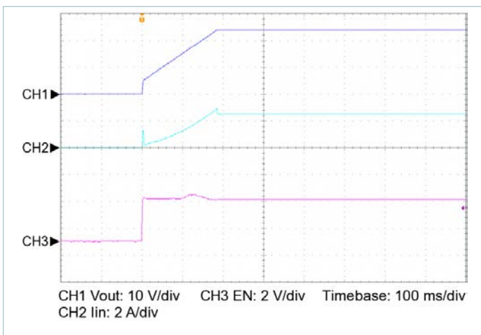
Figure 19 — Start up from EN, V_{IN} = 100\text{V} , C_{OUT\_EXT} = 20000\mu\text{F} , R_{LOAD} = 2.400\Omega
