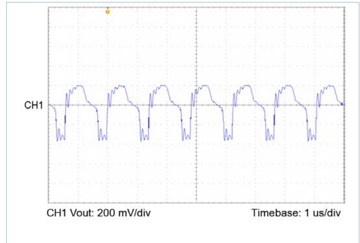
Figure 18 — Output voltage ripple, V_{IN} = 100\text{V} , V_{OUT} = 24.0\text{V} , C_{OUT\_EXT} = 1000\mu\text{F} , R_{LOAD} = 2.400\Omega
