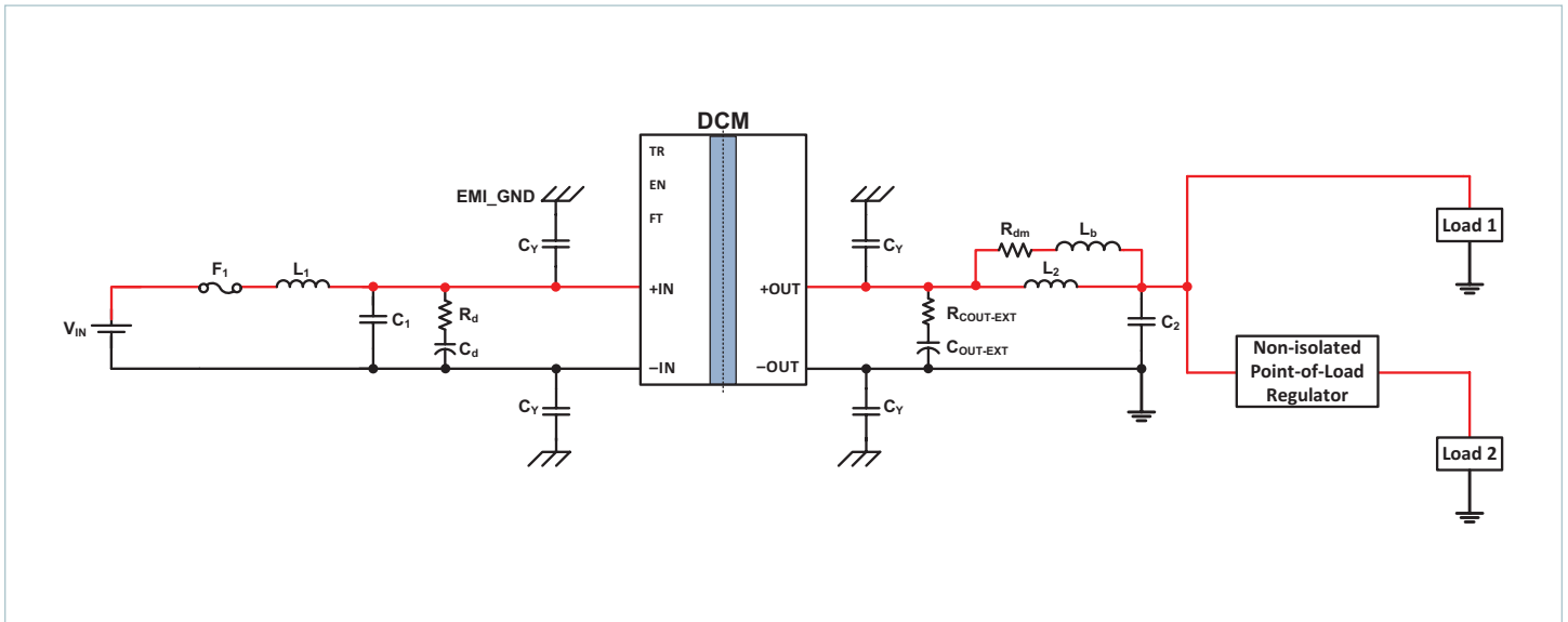
Typical application 1: single DCM3623xA5N31B4y7z to a non-isolated regulator and direct to load
