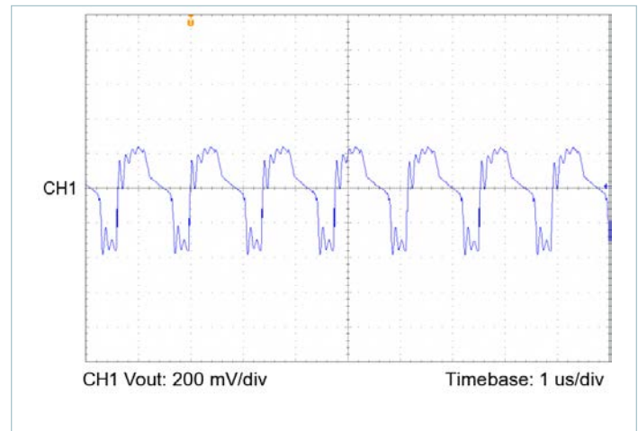
Figure 18 — Output voltage ripple, V_{IN} = 100\text{V} , V_{OUT} = 28.0\text{V} , C_{OUT\_EXT} = 1000\mu\text{F} , R_{LOAD} = 3.256\Omega
