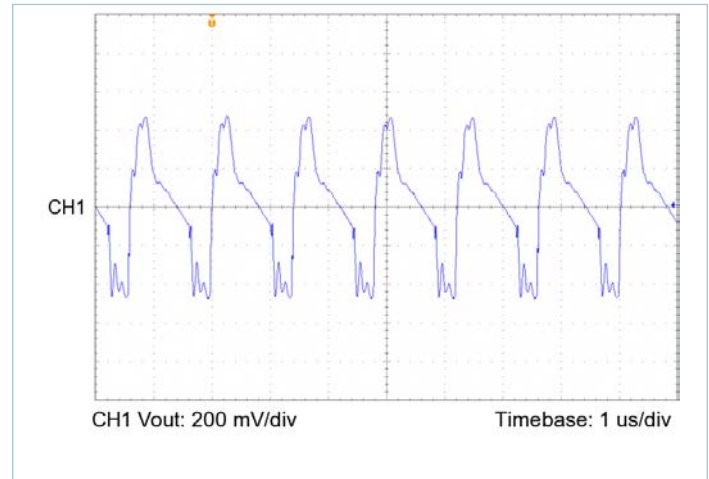
Figure 18 — Output voltage ripple, V_{IN} = 100\text{V} , V_{OUT} = 48.0\text{V} , C_{OUT\_EXT} = 200\mu\text{F} , R_{LOAD} = 9.600\Omega
