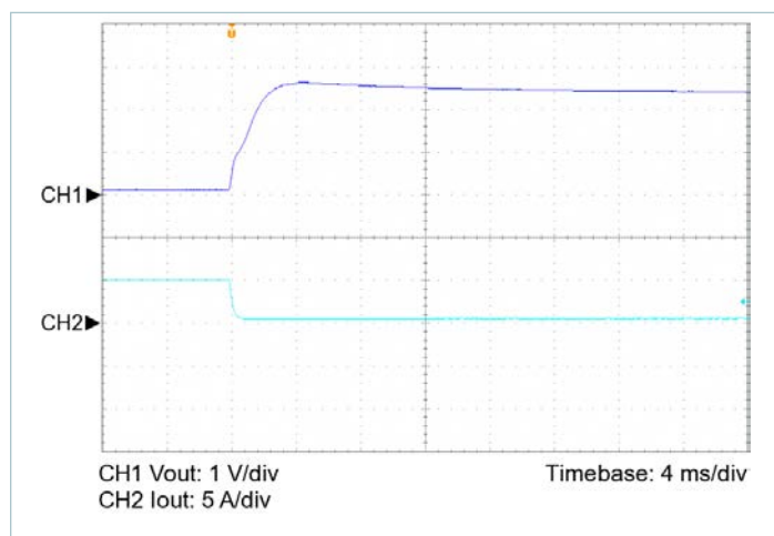
Figure 7 — 100 – 10% load transient response, V_{IN} = 100\text{V} , nominal trim, C_{OUT\_EXT} = 200\mu\text{F}
