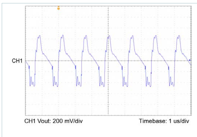
Figure 22 — Output voltage ripple, V_{IN} = 100\text{V} , V_{OUT} = 48.0\text{V} , C_{OUT\_EXT} = 200\mu\text{F} , R_{LOAD} = 9.600\Omega
