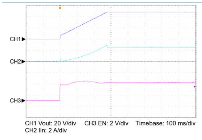
Figure 20 — Start up from EN, V_{IN} = 100\text{V} , C_{OUT\_EXT} = 4000\mu\text{F} , R_{LOAD} = 9.600\Omega
