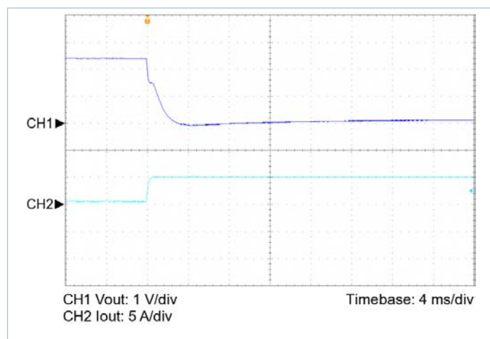
Figure 8 — 10 – 100% load transient response, V_{IN} = 100\text{V} , nominal trim, C_{OUT\_EXT} = 200\mu\text{F}
