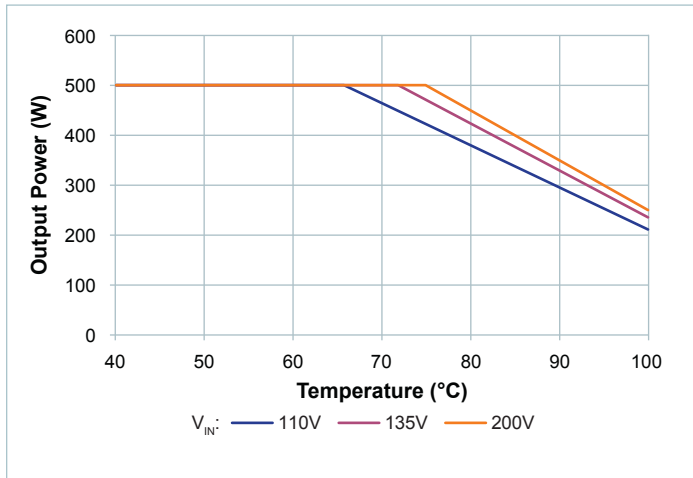
Figure 2 — Thermal specified operating area; max output power vs. case temp, single unit at minimum full-load efficiency; bottom and leads at temperature
