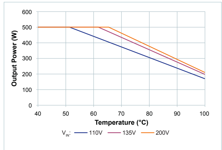
Figure 5 — Thermal specified operating area; max output power vs. case temp, single unit at minimum full-load efficiency; top only at temperature
