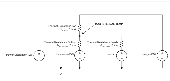
Figure 20 — Double-side cooling and leads thermal model
