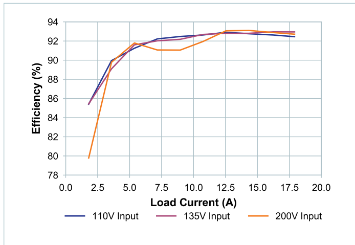
Figure 16 — Efficiency vs. load at T_{CASE} = 25^\circ\text{C} , nominal trim
