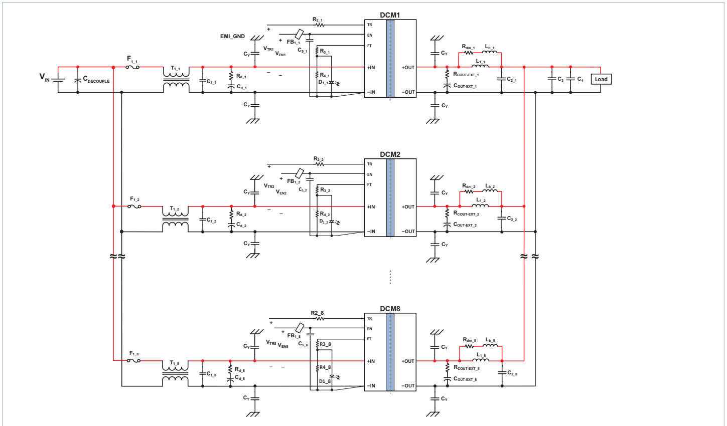
Figure 24 — DCM paralleling configuration circuit 2
