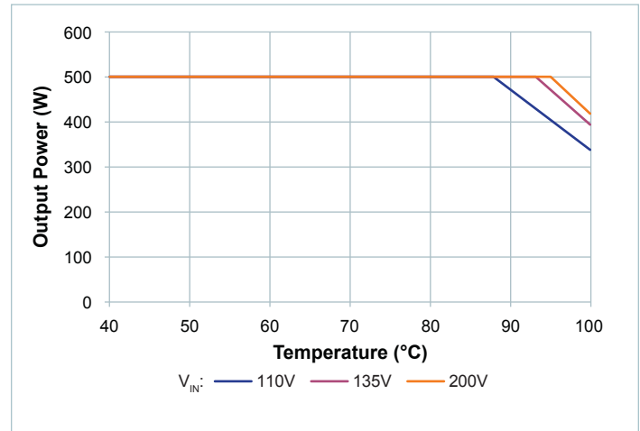
Figure 3 — Thermal specified operating area; max output power vs. case temp, single unit at minimum full-load efficiency; top, bottom and leads at temperature
