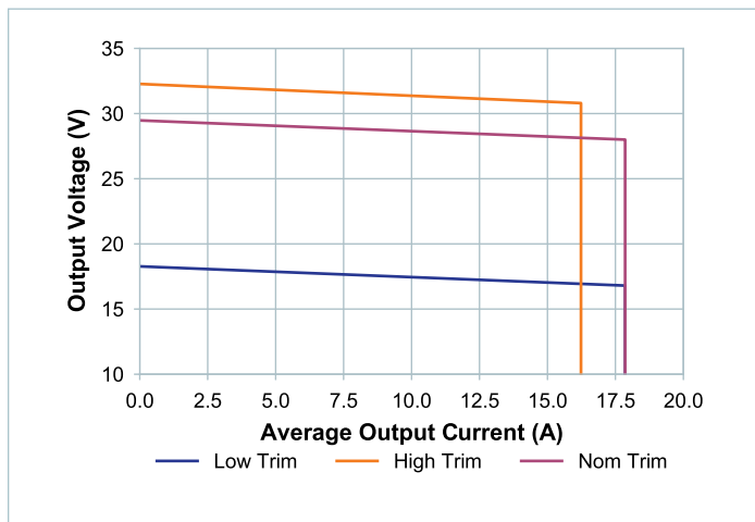
Figure 1 — Electrical specified operating area (does not include light-load boosting)
