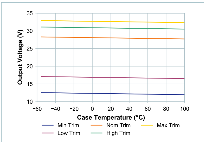
Figure 8 — Ideal V_{OUT} vs. case temperature, at full load
