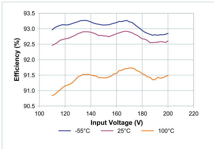
Figure 13 — Full-load efficiency vs. V_{IN} at high trim
