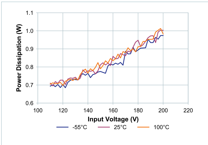
Figure 6 — Disabled power dissipation vs. V_{IN}
