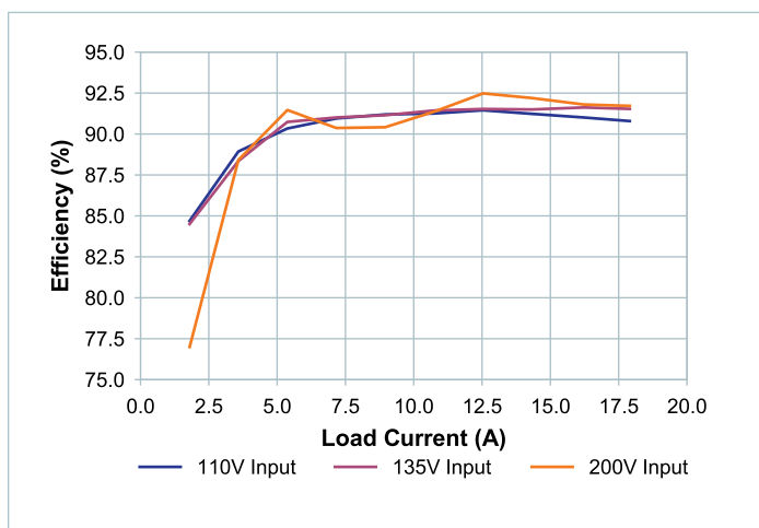
Figure 18 — Efficiency vs. load at T_{CASE} = 100^\circ\text{C} , nominal trim
