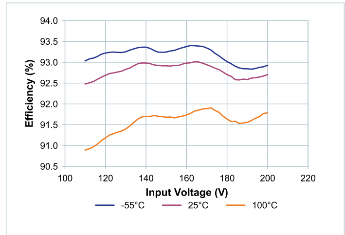
Figure 12 — Full-load efficiency vs. V_{IN} at nominal trim
