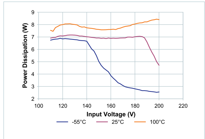
Figure 7 — No-load power dissipation vs. V_{IN} at nominal trim
