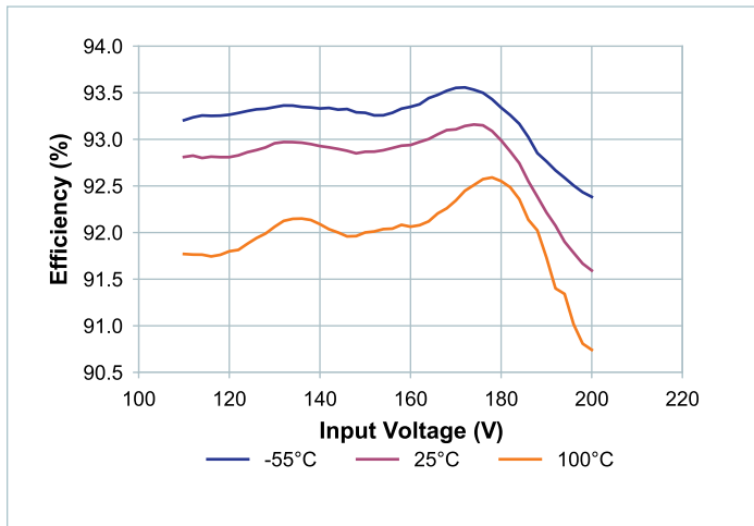
Figure 11 — Full-load efficiency vs. V_{IN} at low trim
