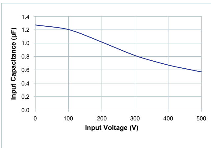
Figure 10 — Effective internal input capacitance vs. applied voltage
