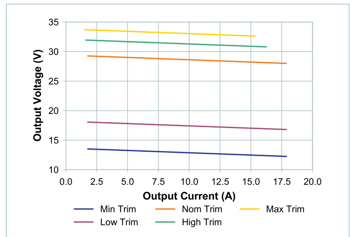
Figure 9 — Ideal V_{OUT} vs. load current, at 25^\circ\text{C} case
