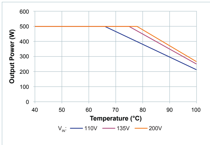
Figure 4 — Thermal specified operating area; max output power vs. case temp, single unit at minimum full-load efficiency; top and leads at temperature
