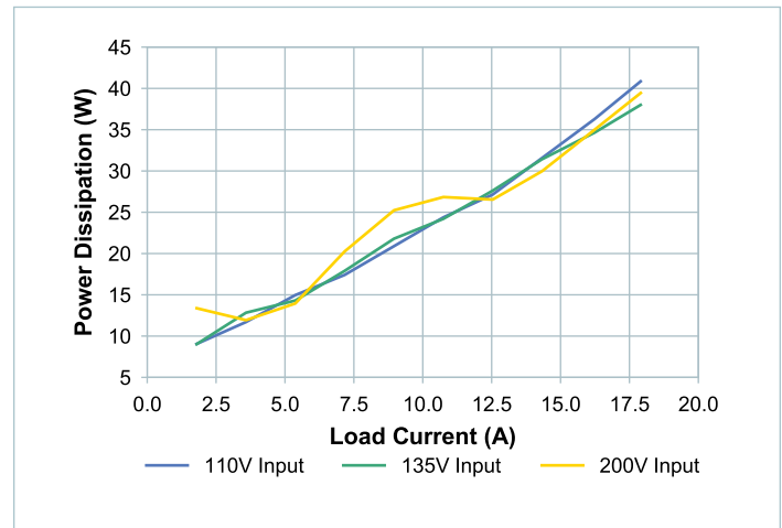
Figure 17 — Power dissipation vs. load at T_{CASE} = 25^\circ\text{C} , nominal trim
