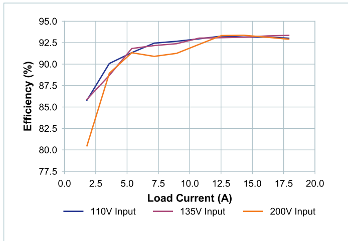
Figure 14 — Efficiency vs. load at T_{CASE} = -55^\circ\text{C} , nominal trim
