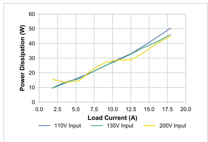
Figure 19 — Power dissipation vs. load at T_{CASE} = 100^\circ\text{C} , nominal trim
