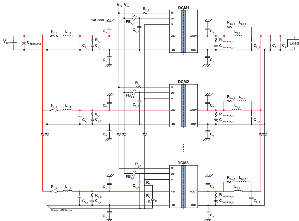
Figure 23 — DCM paralleling configuration circuit 1
