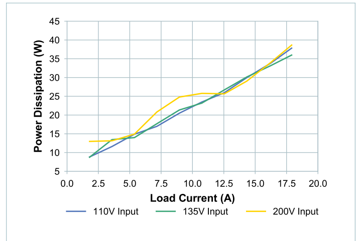
Figure 15 — Power dissipation vs. load at T_{CASE} = -55^\circ\text{C} , nominal trim
