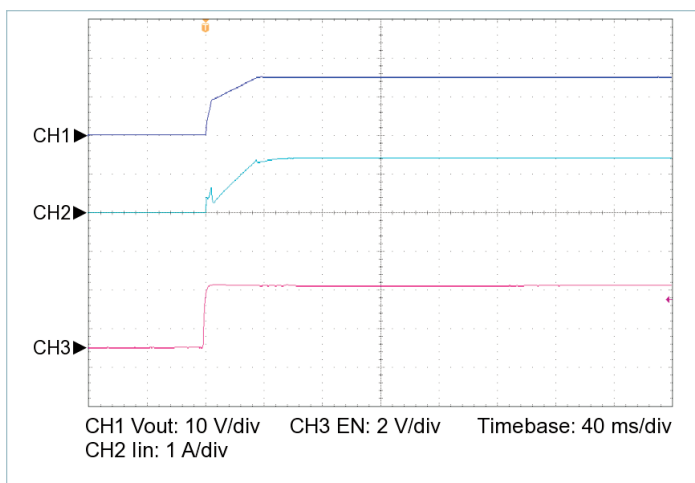
Figure 17 — Startup from EN, V_{IN} = 275\text{ V} , C_{OUT\_EXT} = 10000\text{ }\mu\text{F} , R_{LOAD} = 0.600\text{ }\Omega
