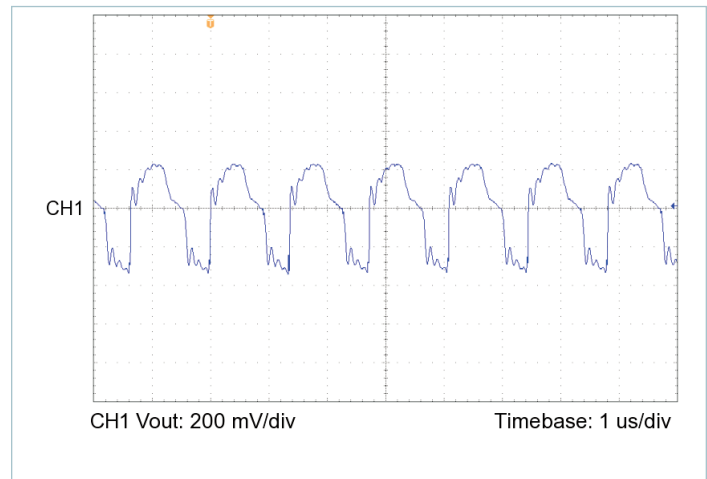
Figure 19 — Output voltage ripple, V_{IN} = 275\text{ V} , V_{OUT} = 15.0\text{ V} , C_{OUT\_EXT} = 1000\text{ }\mu\text{F} , R_{LOAD} = 0.600\text{ }\Omega
