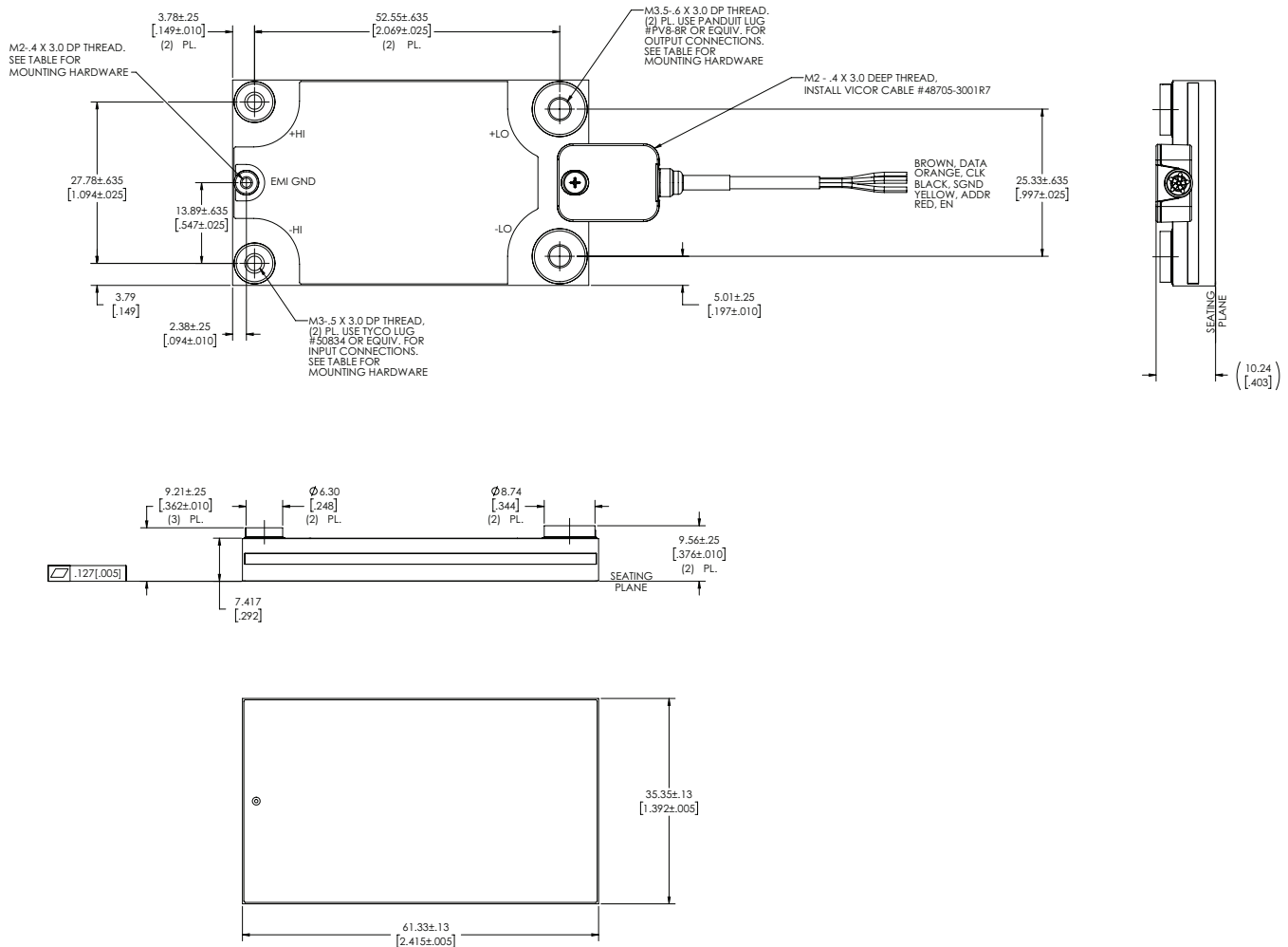
6135 BCM TC7_5 (Reference DWG# 48382 rev 2)
