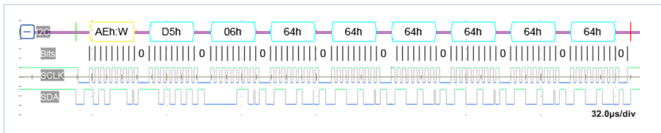
Figure 29 — SET_ALL_THRESHOLDS COMMAND (D5h)_WRITE BLOCK PROTOCOL
