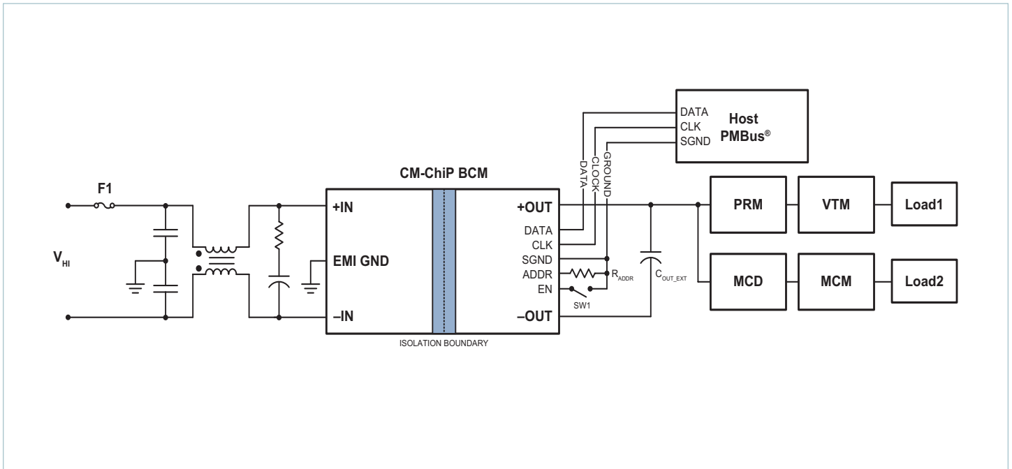
BCM6135CD1E5165TC1 with PRM™ + VTM™ and MCD + MCM™
