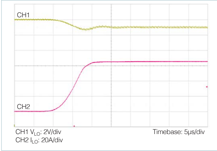
Figure 15 — 0 – 65A transient response, V_{HI} = 384V , C_{LO\_OUT\_EXT} = 0\mu F
