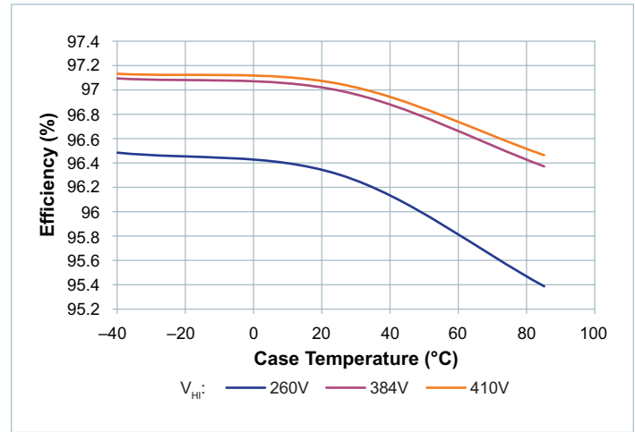
Figure 5 — Full-load efficiency vs. temperature; V_{HI\_DC}
