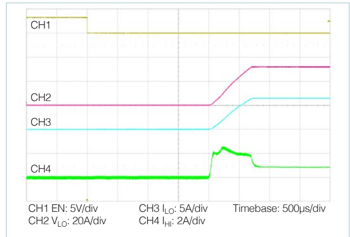
Figure 18 — Start up from application of EN with pre-applied V_{HI} = 384V , 10% I_{LO\_OUT\_DG} , 100% C_{LO\_OUT\_EXT}
