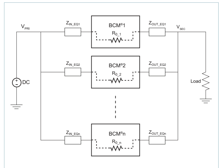
Figure 22 — BCM parallel array
