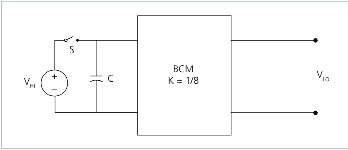
Figure 21 — BCM with high-voltage-side capacitor
