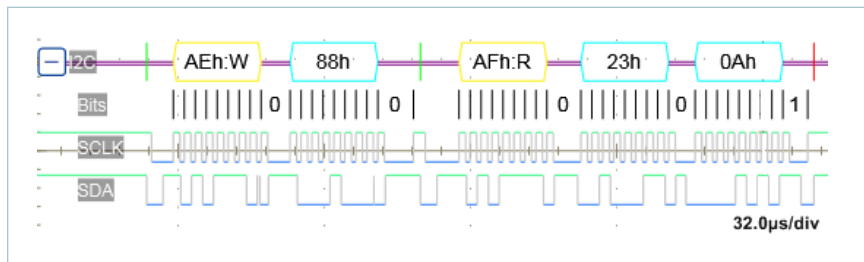
Figure 28 — MFR_VIN_MIN COMMAND (88h)_READ WORD PROTOCOL
