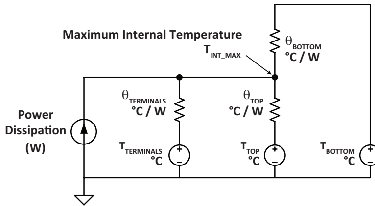
Figure 23 — Two-sided cooling thermal model
