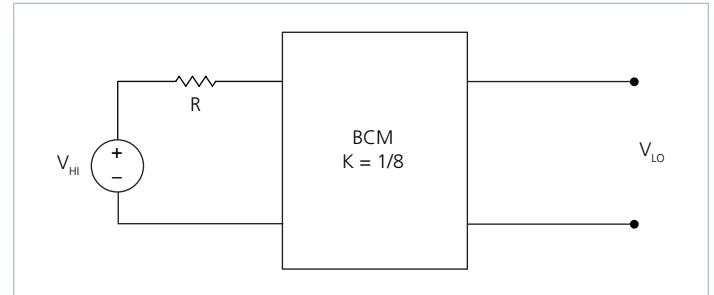
Figure 20 — K = 1/8 BCM with series high-voltage-side resistor
