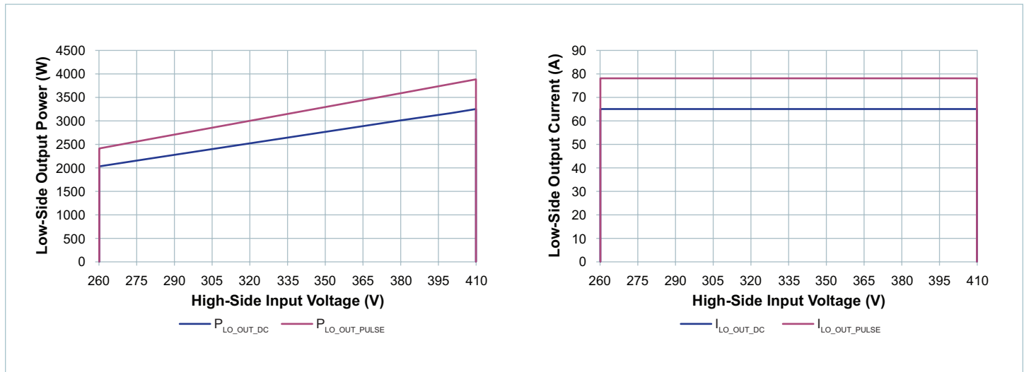
Figure 2 — Specified electrical operating area using rated R_{LO\_HOT}
