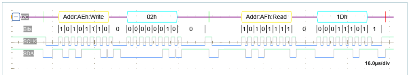
Figure 26 — ON_OFF_CONFIG COMMAND (02h), READ BYTE PROTOCOL
