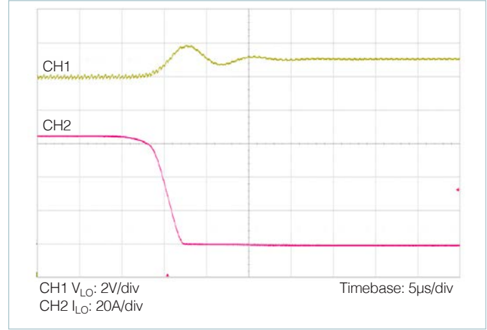
Figure 16 — 65 – 0A transient response, V_{HI} = 384V , C_{LO\_OUT\_EXT} = 0\mu F
