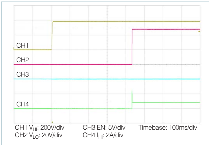
Figure 17 — Start up from application of V_{HI} = 384V , 10% I_{LO\_OUT\_DG} , 100% C_{LO\_OUT\_EXT}
