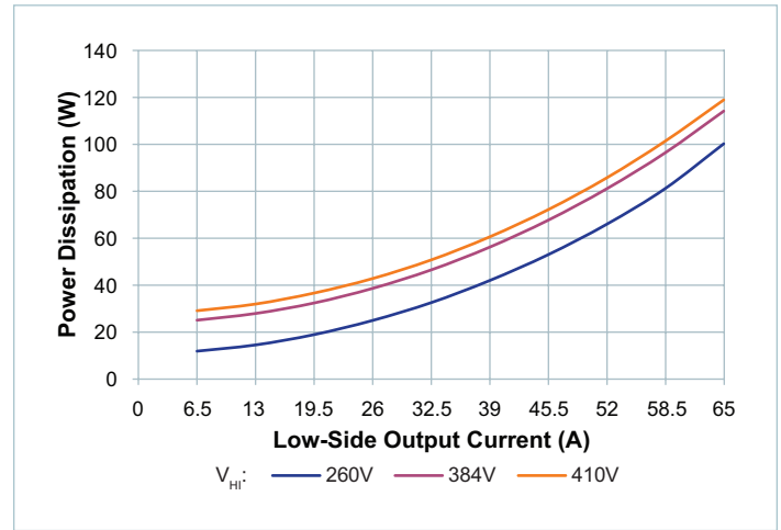
Figure 11 — Power dissipation at T_{CASE} = 85^{\circ}\text{C}
