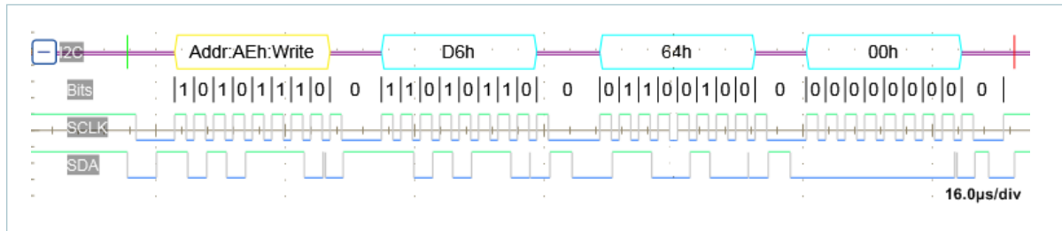
Figure 27 — TON_DELAY COMMAND (D6h)_WRITE WORD PROTOCOL
