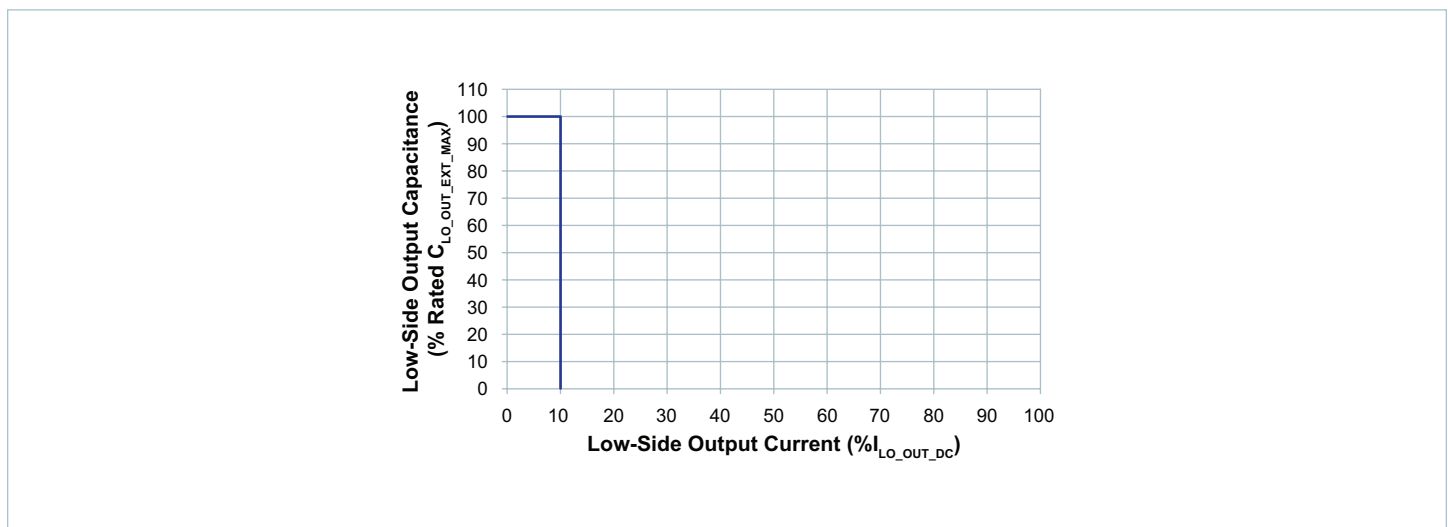
Figure 3 — Specified high-side start up into load current and external capacitance
