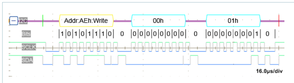
Figure 25 — PAGE COMMAND (00h), WRITE BYTE PROTOCOL
