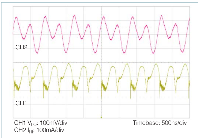
Figure 14 — Full-load low-side voltage and high-side current ripple; no external C_{LO\_OUT\_EXT}
