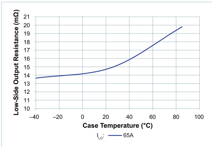
Figure 12 — R_{LO} vs. temperature; nominal V_{HI\_DC} , I_{LO\_DC} = 65\text{A}
