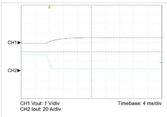
Figure 7 — 100 – 10% load transient response, V_{IN} = 300\text{V} , nominal trim, C_{OUT\_EXT} = 1000\mu\text{F}
