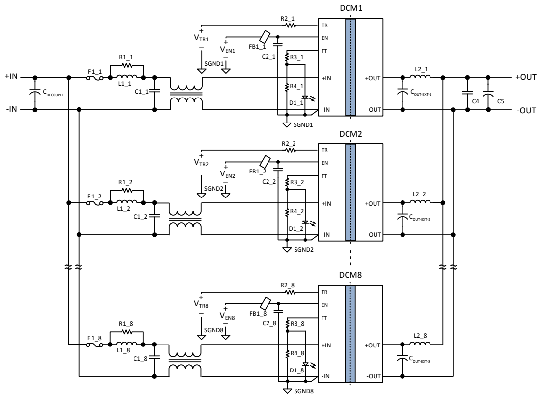
Figure 27 — DCM paralleling configuration circuit 2
