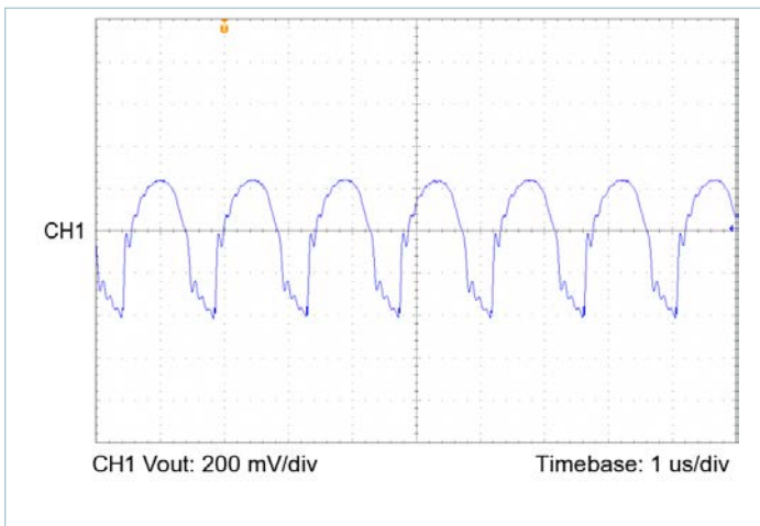
Figure 22 — Output voltage ripple, V_{IN} = 300\text{V} , V_{OUT} = 12.0\text{V} , C_{OUT\_EXT} = 1000\mu\text{F} , R_{LOAD} = 0.359\Omega
