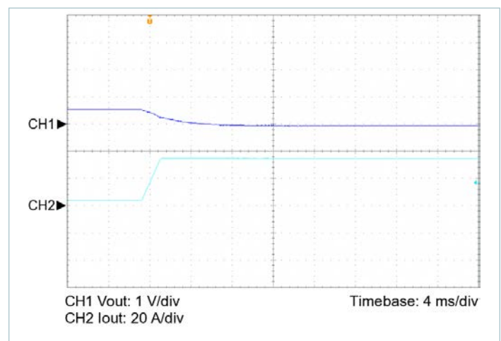
Figure 8 — 10 – 100% load transient response, V_{IN} = 300\text{V} , nominal trim, C_{OUT\_EXT} = 1000\mu\text{F}
