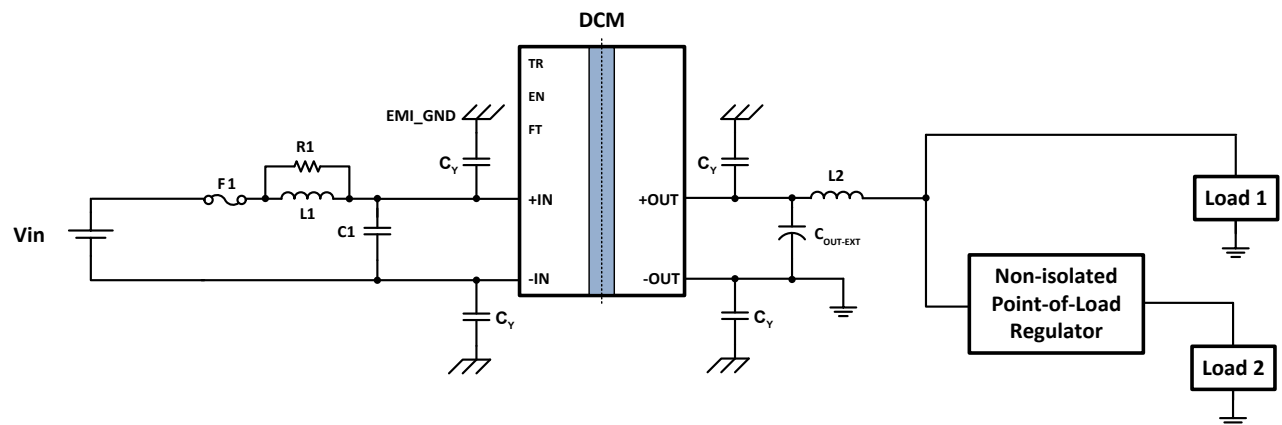
Typical application 2: single DCM4623TD2J13D0T01, to a non-isolated regulator, and direct to load
