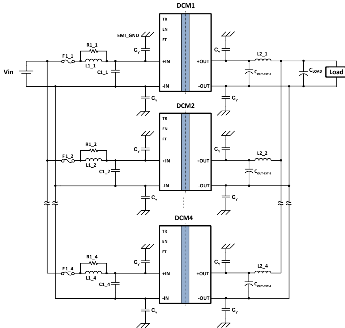
Typical application 1: DCM4623TD2J13D0T01 in an array of four units
