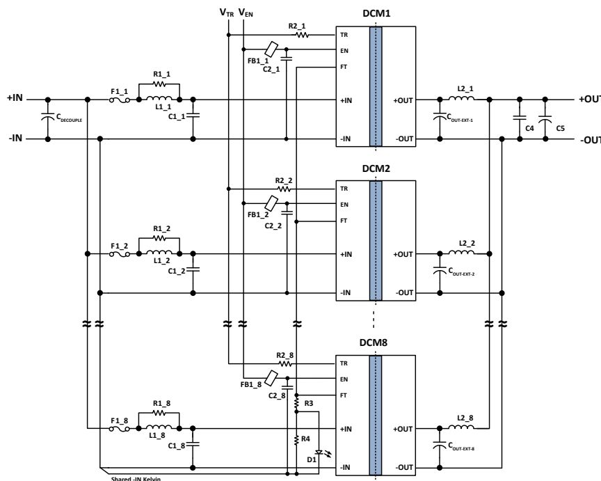
Figure 26 — DCM paralleling configuration circuit 1
