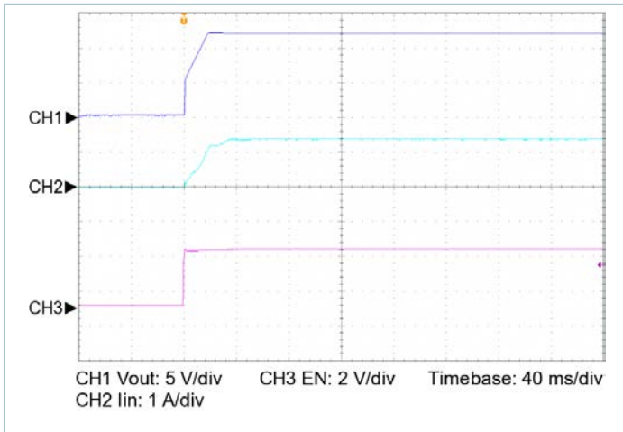
Figure 20 — Start up from EN, V_{IN} = 300\text{V} , C_{OUT\_EXT} = 10000\mu\text{F} , R_{LOAD} = 0.359\Omega
