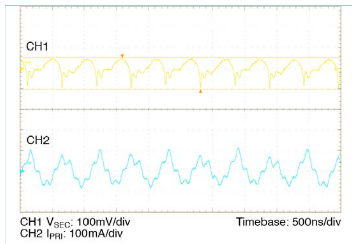
Figure 14 — Full-load secondary voltage and primary current ripple, 2700\mu\text{F } C_{PRI\_IN\_EXT} ; no external C_{SEC\_OUT\_EXT} . Board-mounted module, scope setting: 20MHz analog BW
