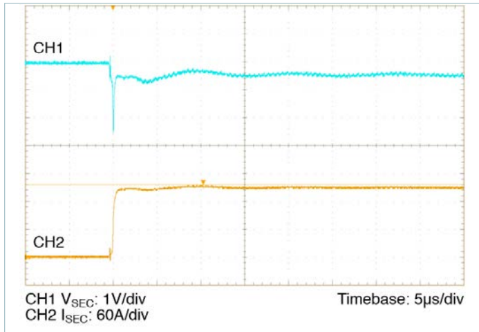
Figure 15 — 0 – 150A transient response:
