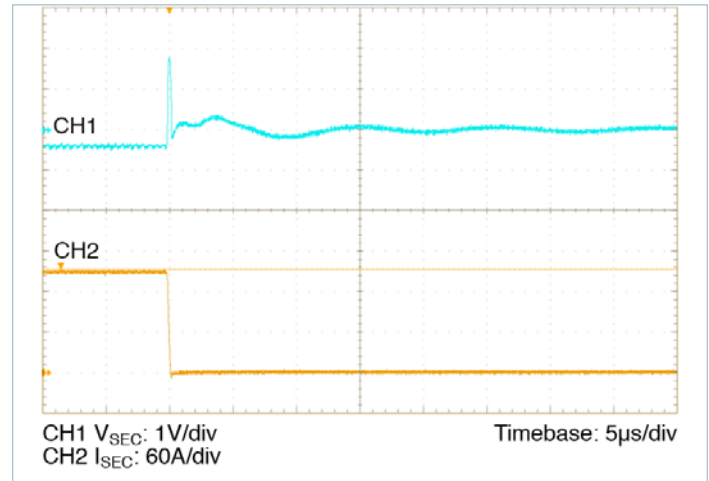
Figure 16 — 150 – 0A transient response:
