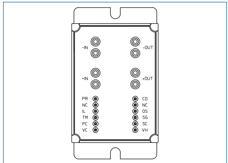
Figure 14 — VI Brick PRM pin configuration (viewed from pin side).
